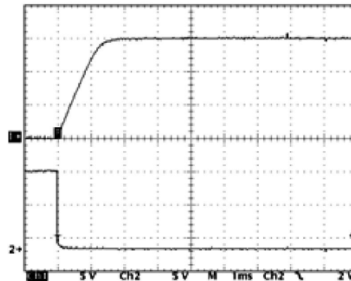
Typical Start-Up Wave Form
