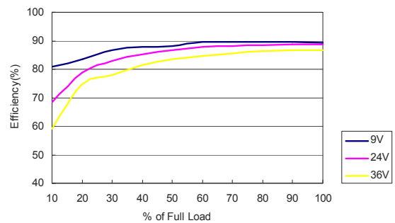
MKWI40-24D12 Efficiency vs Load Current
