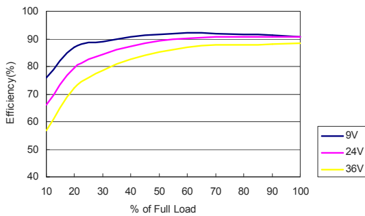
MKWI40-24S033 Efficiency vs Load Current
