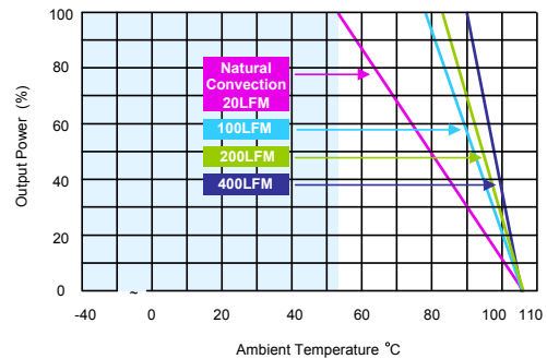
MKWI40-24S12, MKWI40-24S15 Derating Curve with Heatsink
