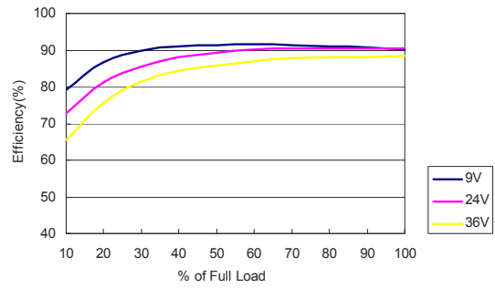
MKWI40-24S05 Efficiency vs Load Current
