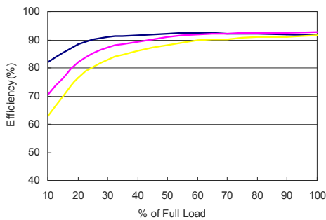
MKWI40-48S24 Efficiency vs Load Current
