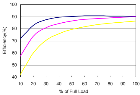
MKWI40-48S033 Efficiency vs Load Current
