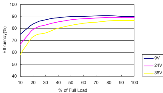
MKWI40-24S24 Efficiency vs Load Current
