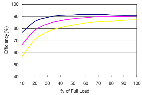
MKWI40-48S05 Efficiency vs Load Current
