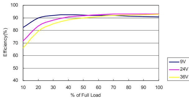
MKWI40-24S24 Efficiency vs Load Current
