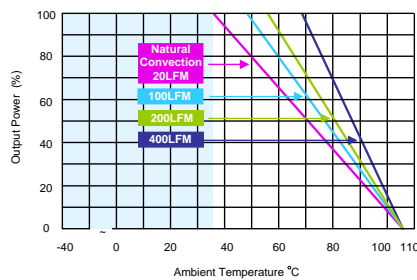
MTQZ75-72S05, MTQZ75-110S05 Derating Curve without Heatsink
