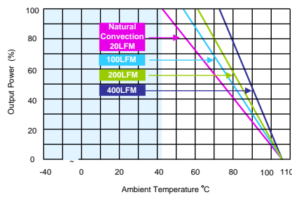
MTQZ75-110S24 Derating Curve without Heatsink
