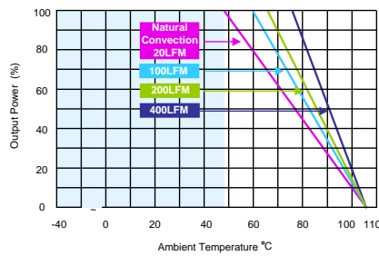
MTQZ75-110S12, MTQZ75-110S15, MTQZ75-72S24 Derating Curve without Heatsink
