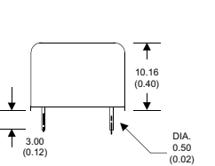
16 Pin DIL Package Nickel-Coated Copper
