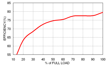
FKC05-48S05 Efficiency vs. Output Load
