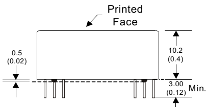
For "M" Case 24 Pin DIL Package Nickel-Coated Copper
