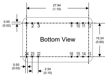
For "M" Case 24 Pin DIL Package Nickel-Coated Copper
