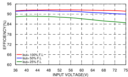
HAE100-48S05 Efficiency vs. Input Voltage
