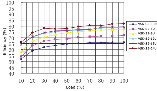
2. efficiency vs. output power (Vin=220Vac)
