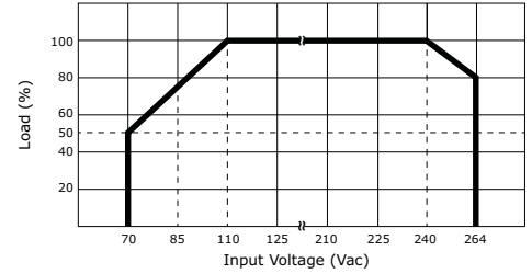
2. output power vs. input voltage
