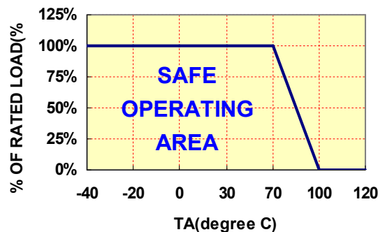
TEMPERATURE DERATING
