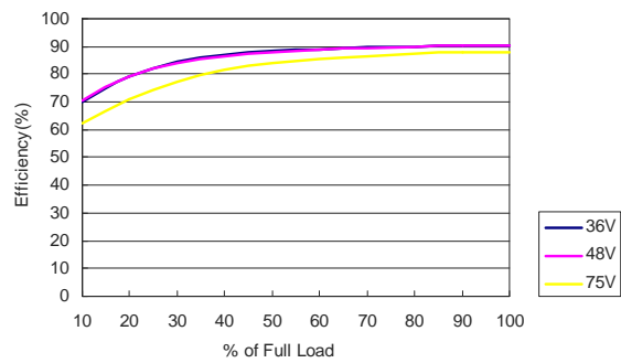
MKW40-48S15 Efficiency vs Load Current
