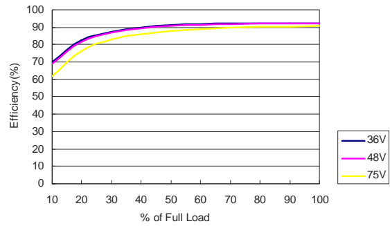
MKW40-48S05 Efficiency vs Load Current
