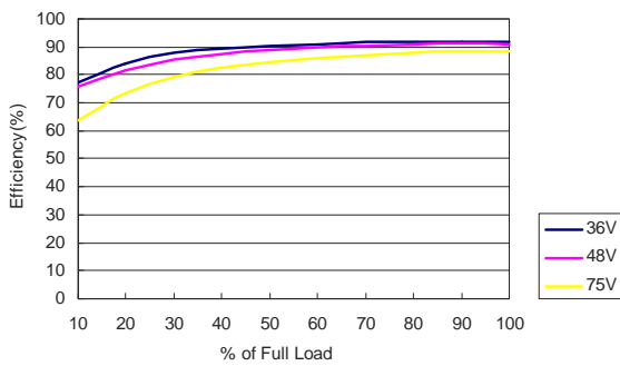
MKW40-48S12 Efficiency vs Load Current
