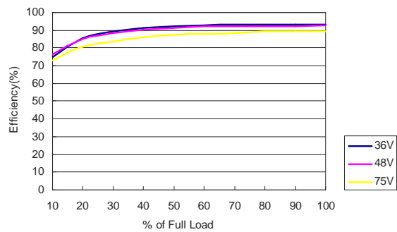
MKW40-48S05 Efficiency vs Load Current
