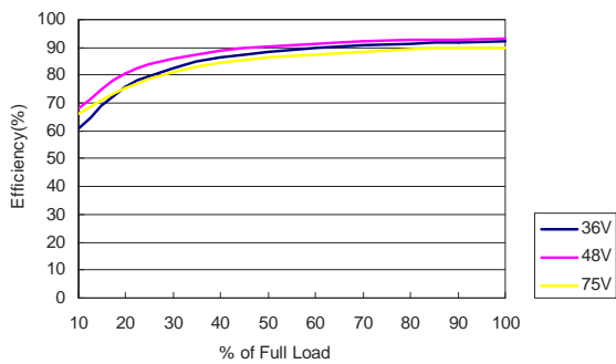
MKW40-48S033 Efficiency vs Load Current
