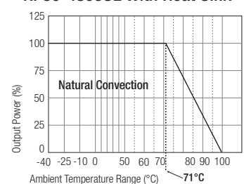
RP30-4805SE With Heat Sink
